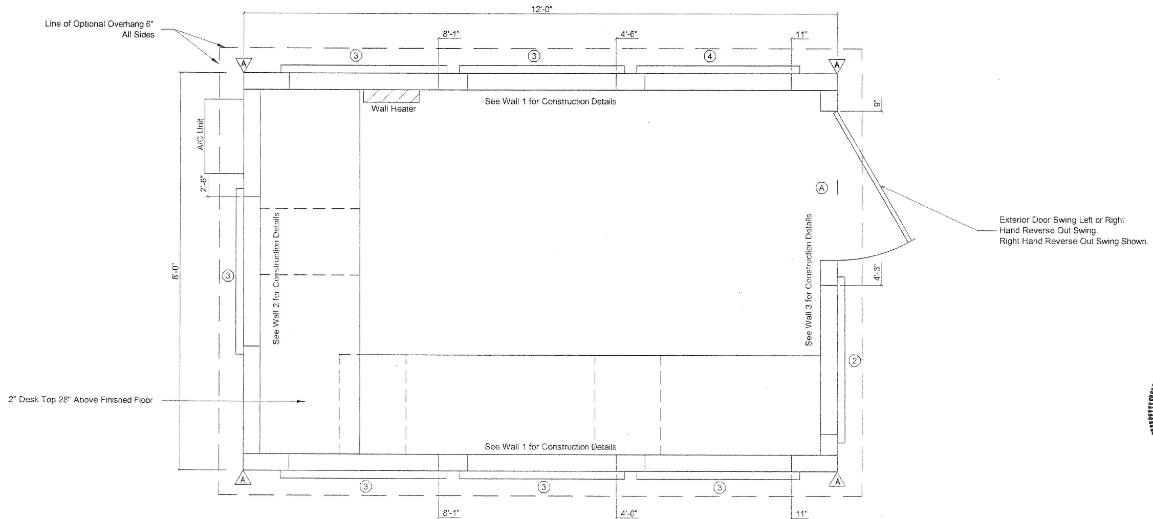
PLAN A FLOOR PLAN
