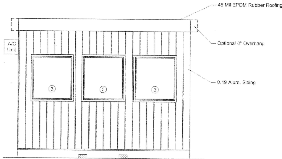
FRONT ELEVATION- PLAN A SCALE: 1/4" = 1'-0"
